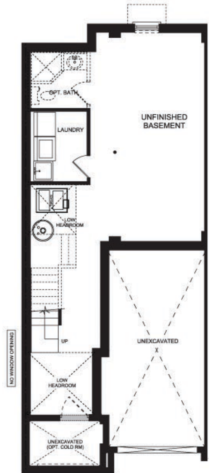
BASEMENT PLAN
