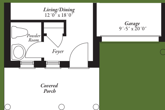
Partial First Floor Plan Elevation B
