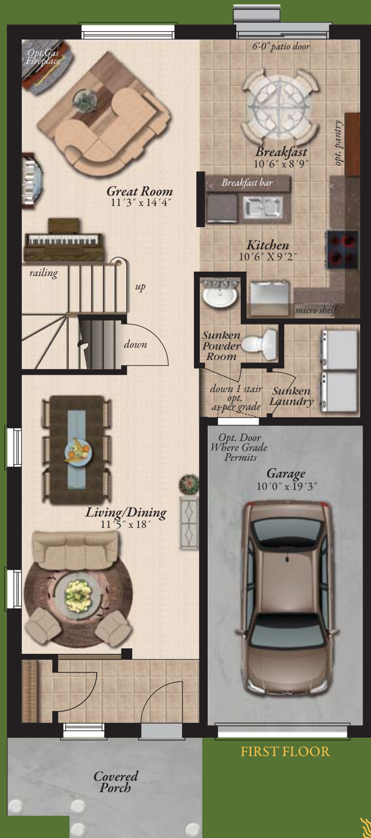
Partial Ground Floor Plan Elevation B
