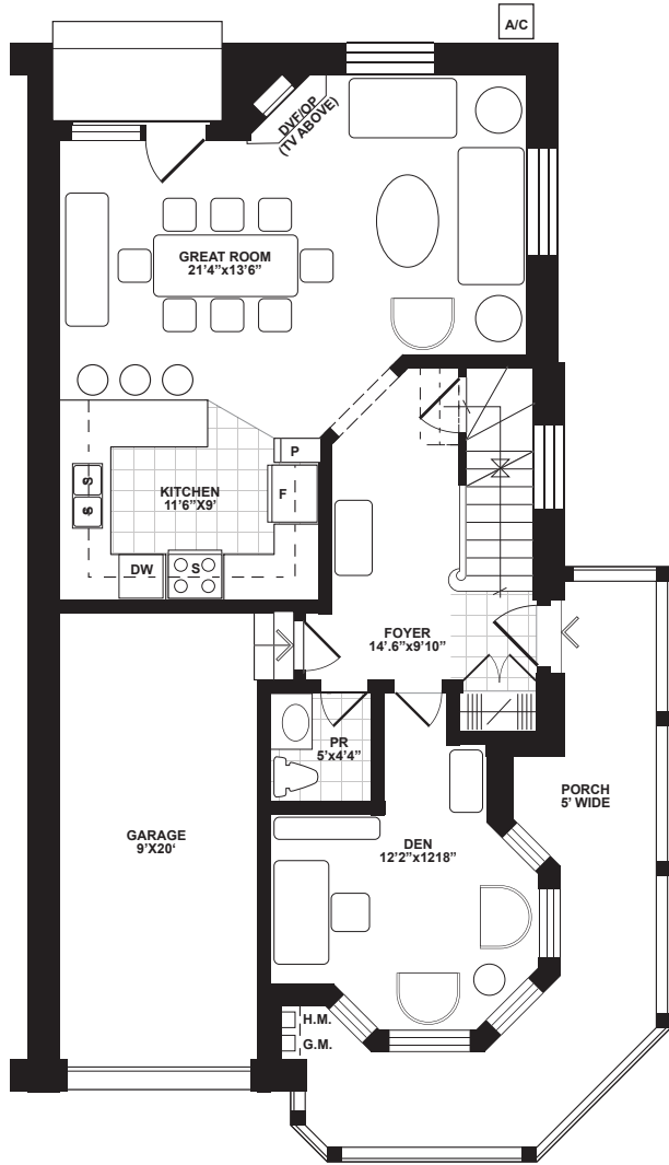
FIRST FLOOR
